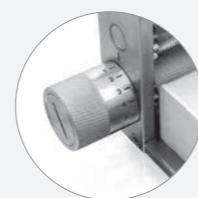
Graft Thickness Adjustment (0-1,5 mm)
